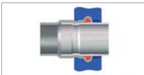
■ Pressed joint.
