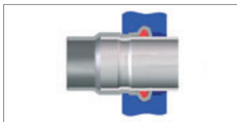
■ Pressed joint.
